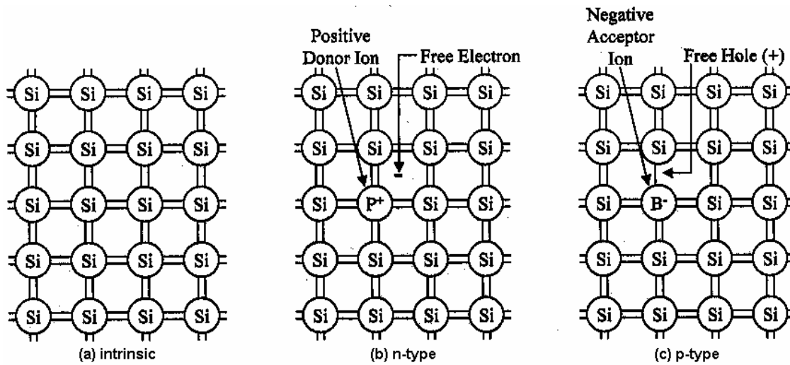
Fig. 2- 7: (a) A two-dimensional lattice structure of a silicon (IV) semiconductor. By adding an atom from group V, phosphorous, an extra electron that is not covalently bonded is introduced into the material (b). This is referred to as an n-type semiconductor. A p-type semiconductor (c) is created by adding atoms of boron, group III, which allows for an extra free hole. (13: 382)
