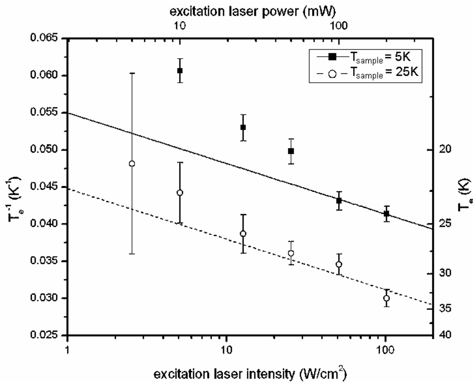
Fig. 4- 20: The plots determining the LO phonon cooling domination range for bulk sample 93-045 at various temperature. The lines represent the 29.1meV LO phonon for InAs_{0.911}Sb_{0.089} .
